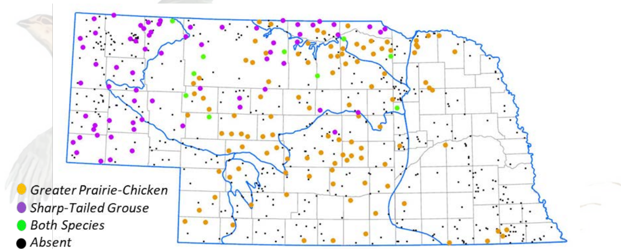
Figure 3. Prairie grouse occurrence during Nebraska's Statewide Prairie Grouse Monitoring Effort, 2020-2022.
